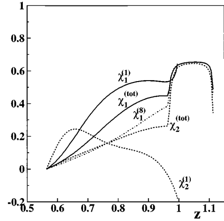
FIG. 2. Energy dependence of the angular coefficient \alpha in e^+e^- \rightarrow \chi_{c1,2} + X at \sqrt{s} = 10.58 GeV: total, color-singlet, and color-octet \chi_{c1} contributions, and total and color-singlet \chi_{c2} contributions.
