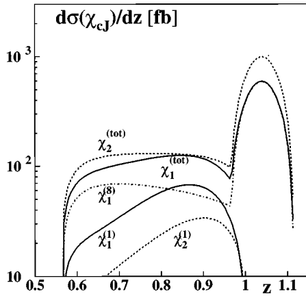
FIG. 1. Energy distribution of \sigma(e^+e^- \rightarrow \chi_{c1,2} + X) at \sqrt{s} = 10.58 GeV: total, color-singlet, and color-octet \chi_{c1} contributions, and total and color-singlet \chi_{c2} contributions. The peak from the e^+e^- \rightarrow c\bar{c}_8(^1S_0, ^3P_J) + g processes at large z has been smeared over a range of width \sim v^2 . In a physical process such a smearing follows from the energy transfer in the non-perturbative transition.
